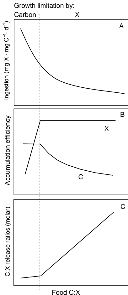
Fig. 2. Predicted trends in ingestion (A), accumulation efficiency (B), and C:X release ratios from (C) a homeostatic consumer eating food of differing C:X ratio where X is any non-C element. Here accumulation efficiency represents the fraction of element incorporated into growth relative to the amount ingested. The shapes of these predictions are based on modified equations from the consumer growth model presented in Sterner (1997) and under the condition of high food quantity.
