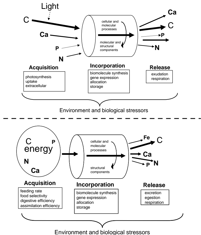
Fig. 1. Conceptual diagram illustrating primary processes regulating the acquisition, incorporation, and release of chemical elements for autotrophs and heterotrophs. Central to these processes are cellular and molecular responses that control the demand for elements in new structural material. These processes feed back into acquisition processes by affecting the production of nutrient uptake and digestive proteins. Disposal is also likely affected by these key cellular processes, as elements acquired in excess are preferentially released. Finally, environmental factors and biological stressors may alter organism physiological stoichiometry by affecting metabolic demands for particular elements.
